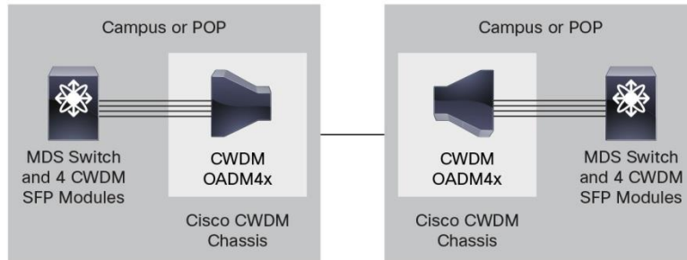
Figure 15. Point-to-Point Architecture (Dual-Fiber Link)
