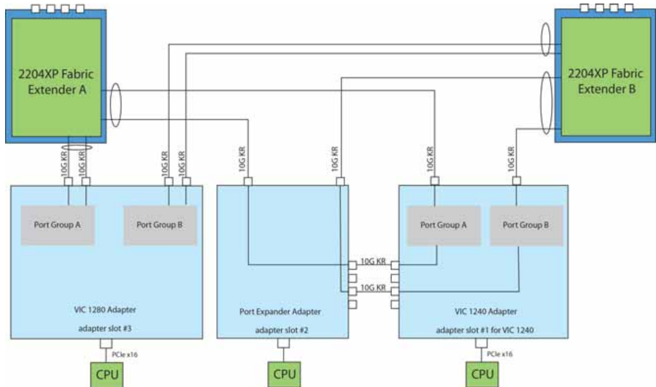
Figure 30 VIC 1240, Port Expander and VIC 1280
