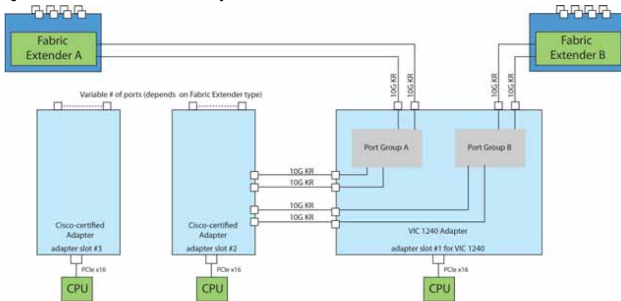
Figure 10 VIC 1240 Connectivity
