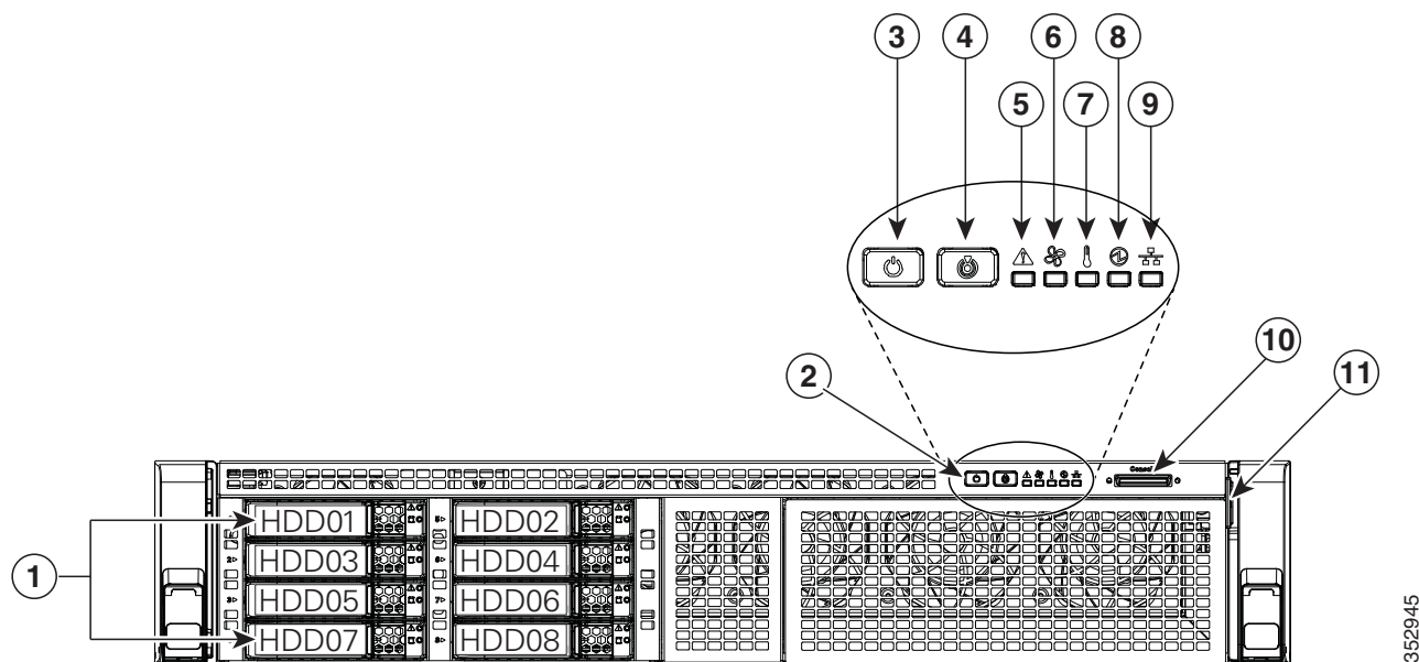
Figure 4 Chassis Front View (8-drive version)
