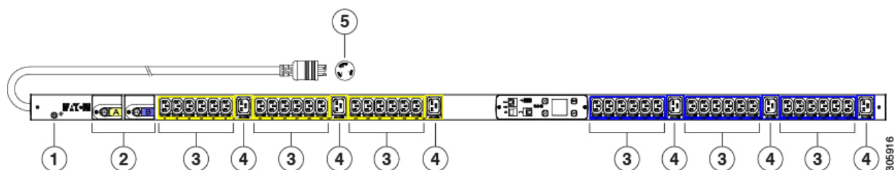
Figure 19 RP208-30M1P-6-36 PDU
